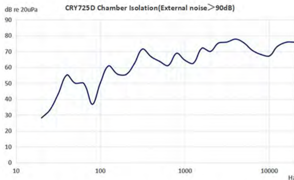
▲ CRY725D Chamber Isolation - Frequency Graph
