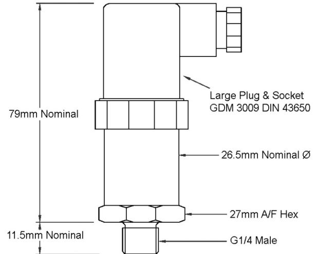
Large Plug & Socket IP65, GDM 3009 DIN 43650
